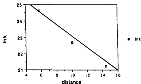
Figure 5. Plot of the rate of electron transfer (data from Figure 3) versus edge to edge distance in the bis-porphyrin series. The slope, \beta = 0.4 \text{ \AA}^{-1} .
