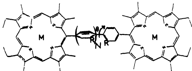
Figure 1. Schematic structures of the polyphenylene-bridged bisporphyrin adducts: M = \text{Fe}^n, \text{Zn}, n = 0, 1, 2 . For the compounds reported here, R = \text{H}, \text{CH}, \text{or } (\text{CH}_2)_2^n(\text{CH}_2)_3 .
